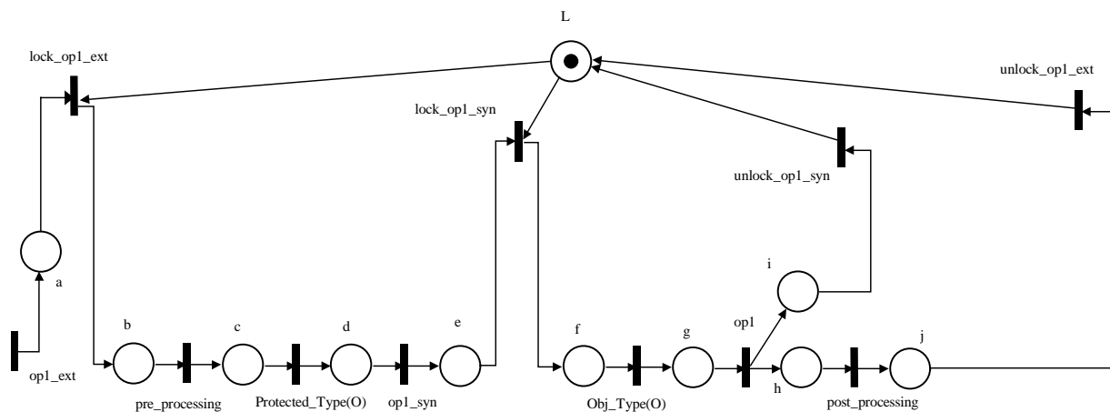
Figure 4. Object.Synchronized.Extended model
