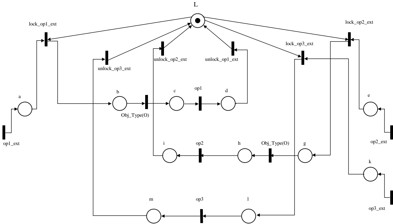
Figure 1. Object.Synchronized.Extended model
