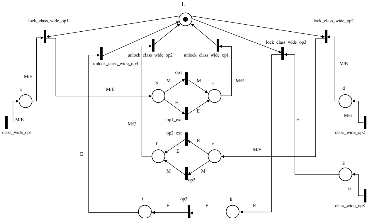
Figure 2. Protected_Object.My_Object.Extended model
